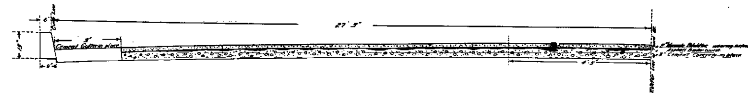
TYPE SECTION OF ONE HALF STREET Scale 1/2 in = 1 ft.
